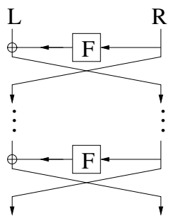
Fig. 1. General Structure of a Feistel cipher
