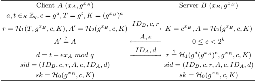
Fig. 4. Jakobsson–Pointcheval MAKEP
