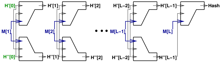
Fig. 3. The Double-Pipe Hash
